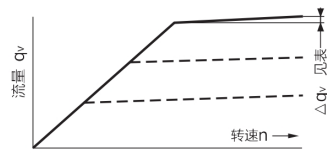
变转速情况下的静态特性曲线 Characteristic curve at variable rotational speed
